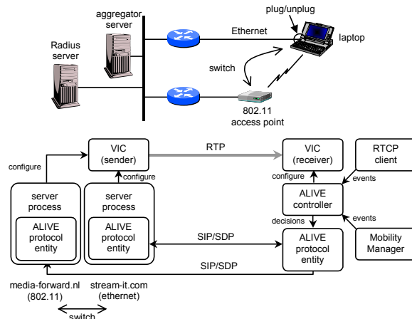
Fig. 9. Testbed
